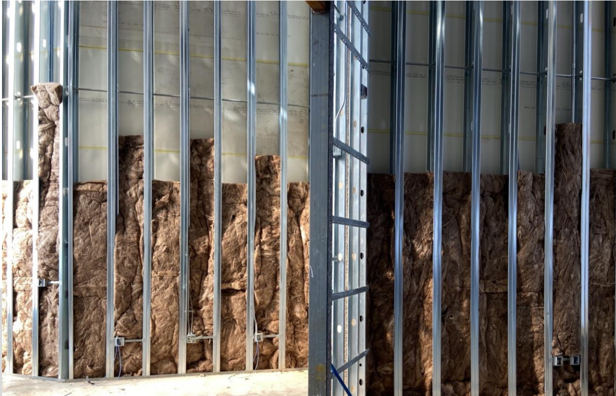
Stuffing Insulation in Media Center Metal Stud Walls
